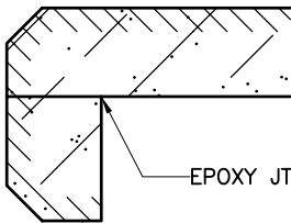
BEVEL WITH APRON
